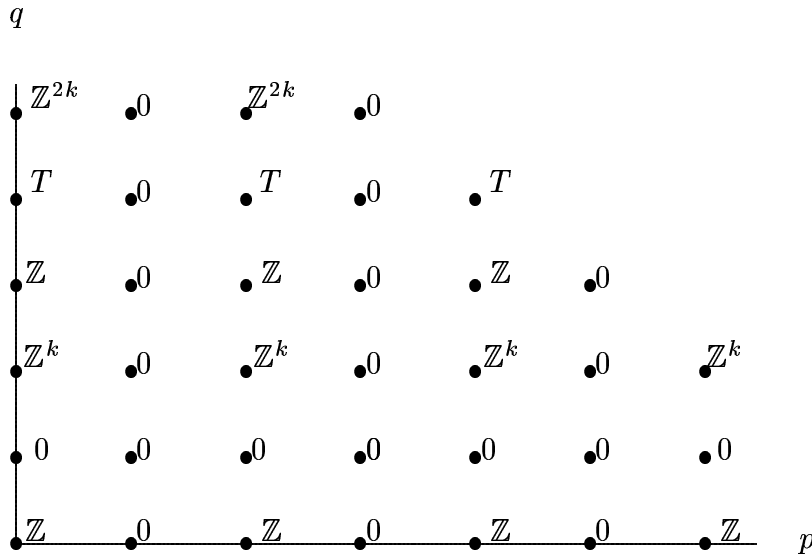
Diagram 5.5: E_2^{p,q} for S^3 \times \mathcal{S} \rightarrow S^3 \star \mathcal{S} \rightarrow BS^1
