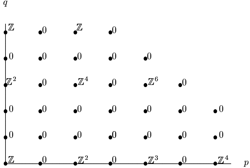
Diagram 5.9: E_2^{p,q} for S^3 \times SU(3) \longrightarrow S^3 \star \mathcal{S}(p_1, p_2, p_3) \longrightarrow BS^1 \times BS^1
